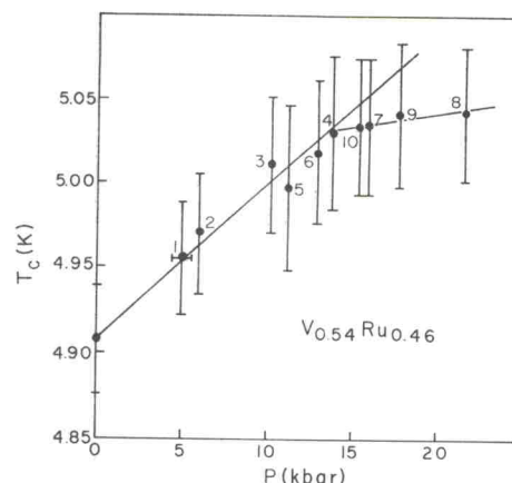
FIG. 4. Pressure dependence of T_c for V_{0.54}Ru_{0.46} .
